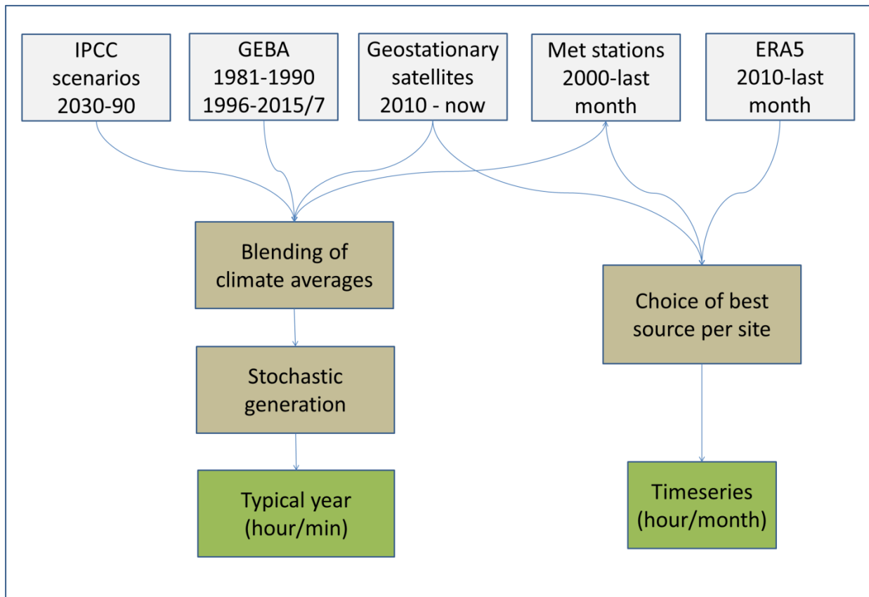
Fig. 3.3.1: Data sources and pathways of data selection and generation: two main paths exist: one for typical years (TMY) and one for ongoing timeseries.
