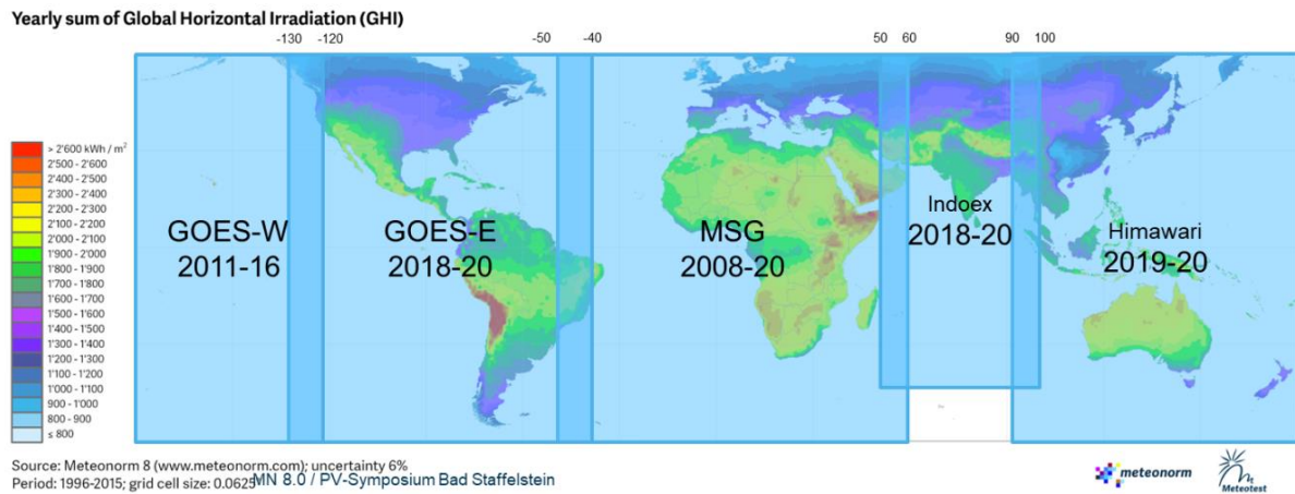
Fig. 3.1.1: Time periods and used geostationary satellite for ongoing timeseries and mapping of climate values.
