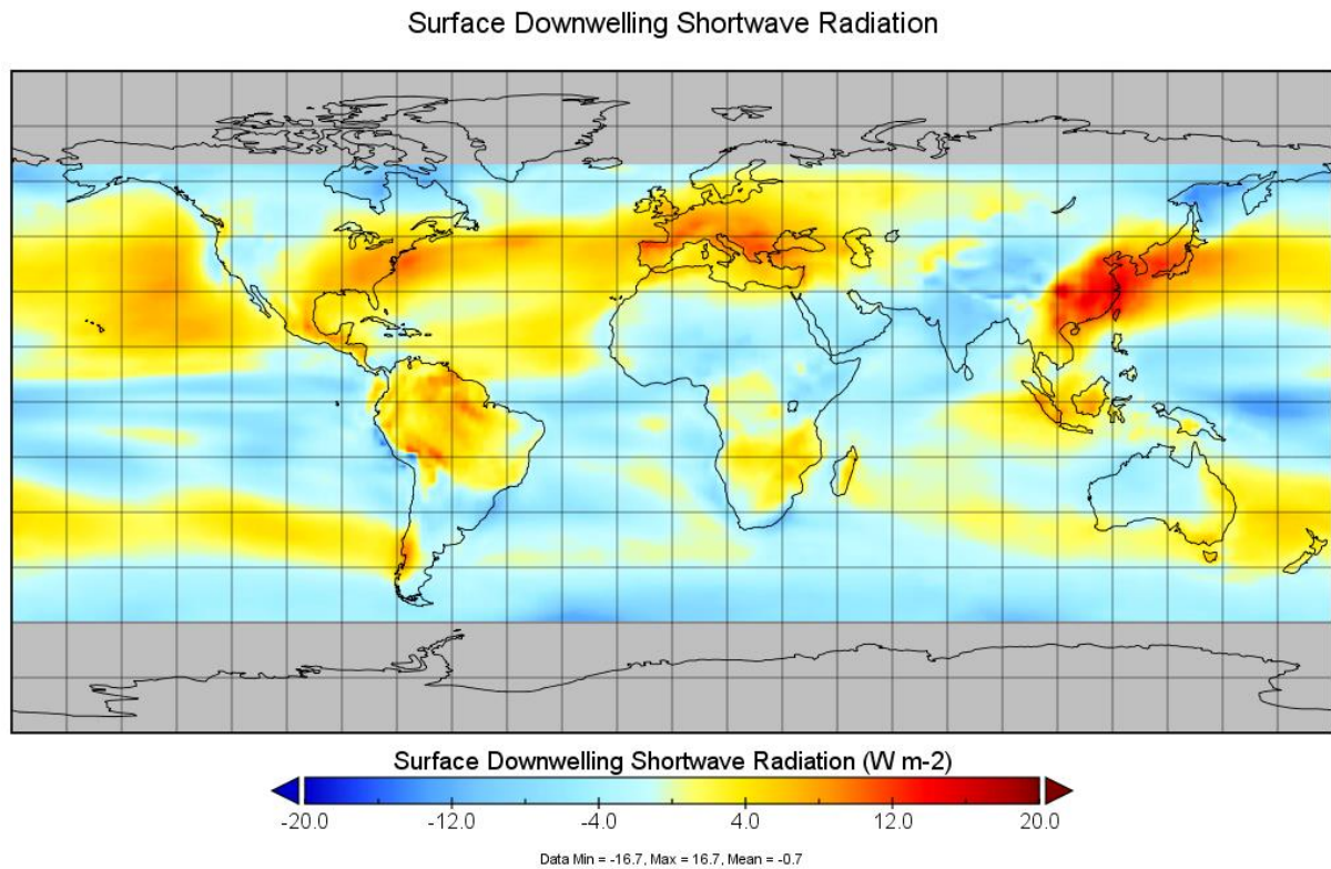
Fig. 3.2.1: Anomalies of global radiation in W/m 2 compared to 1996 - 2015 for the period 2080–2099 with IPCC scenario RCP8.5. Note that the unit is different than in the table above. For a yearly sum in kWh/m 2 , a factor of 8.76 has to be applied.
