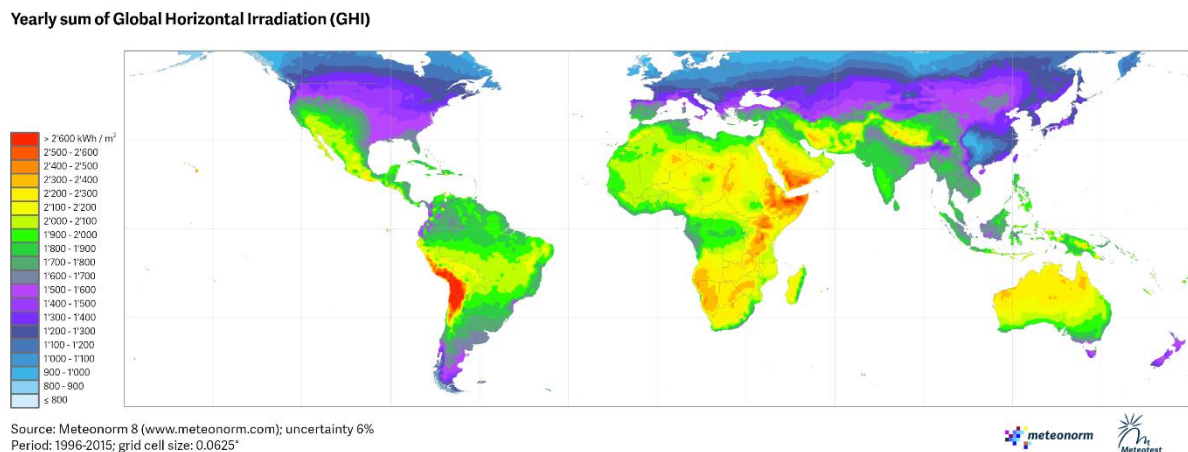
Fig. 3.1.2: Map of yearly sum of global irradiation in kWh/m 2 based on satellite and ground information. Means adapted mainly to the period 1996–2015.
